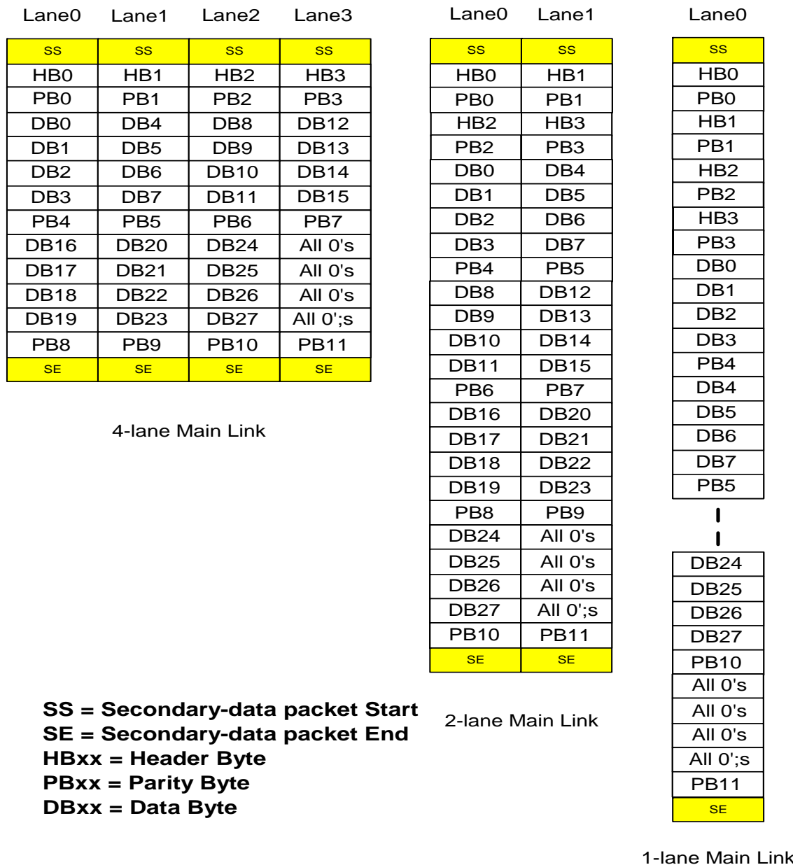
Figure 2-21: InfoFrame Packet
