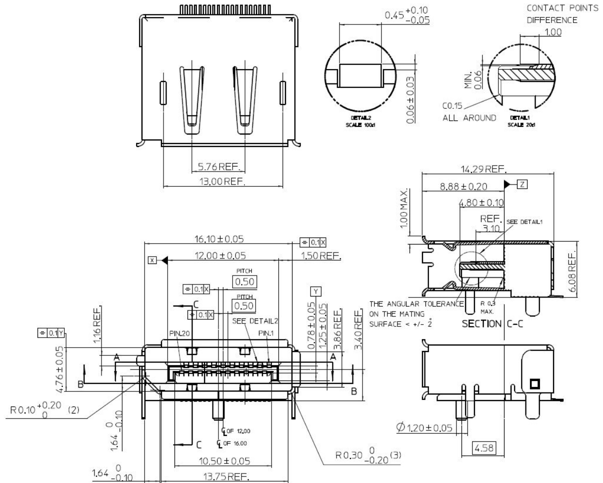
Figure 4-16: DisplayPort External Connector Drawings
