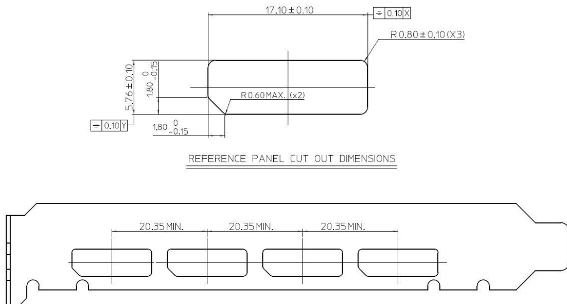
Figure 4-22: Panel Cut Out Reference Dimensions
