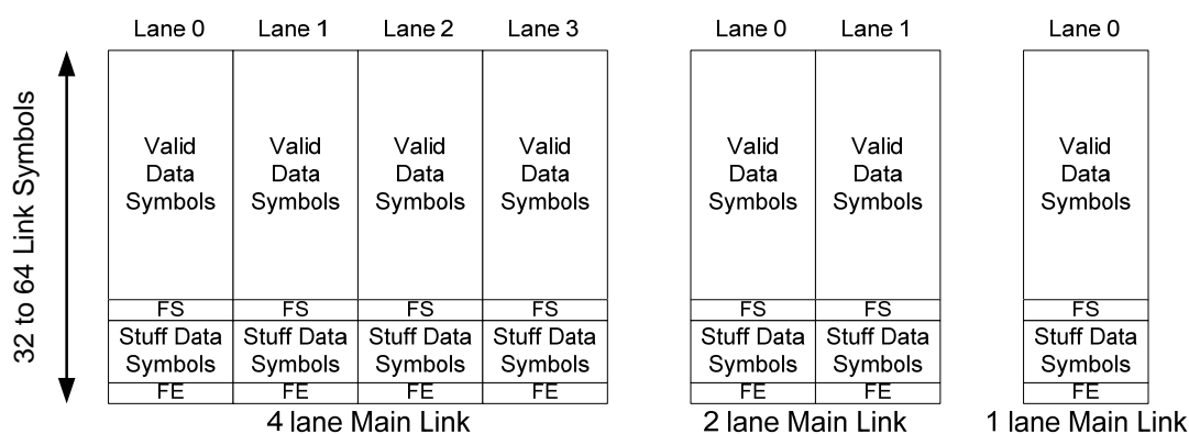
Figure 2-13: Transfer Unit
