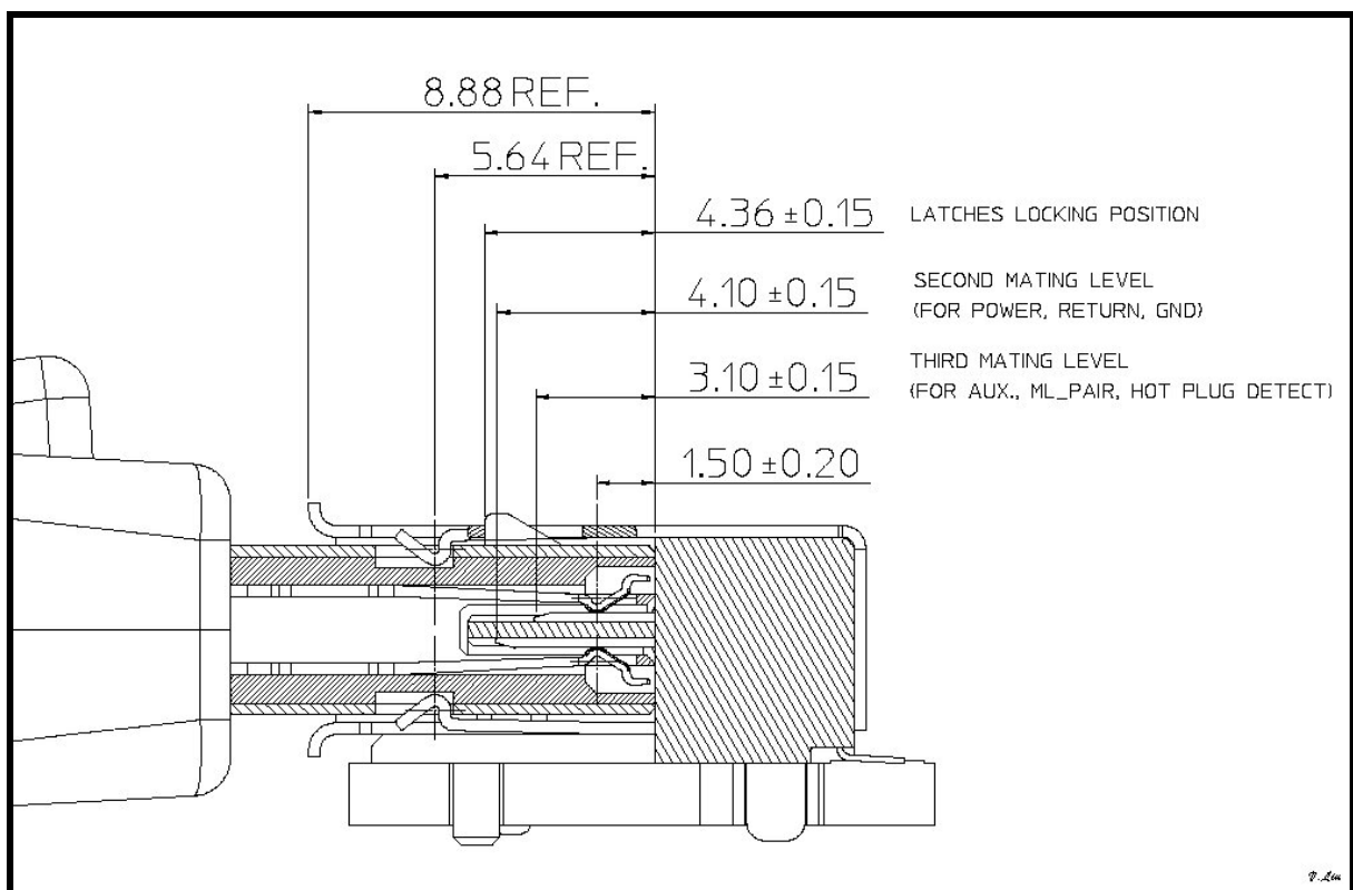
Figure 4-19: Fully-mated Condition for DisplayPort External Connectors
